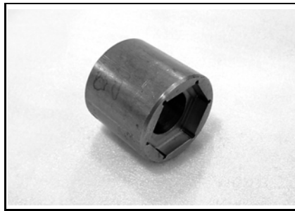
Socket 46 mm machined P/N 529 036 114 Mandatory 991
