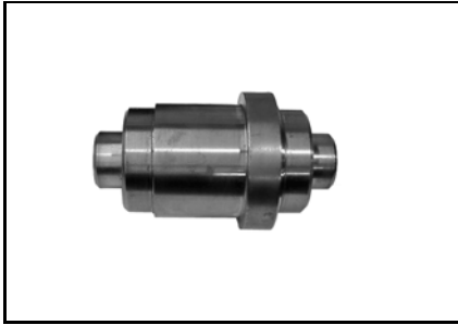
Cranshaft plain bearing tool P/N 529 036 093 Recommended 991 plain bearing
