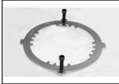
Clutch assembly holder P/N 529 036 133 Mandatory 991 engines
