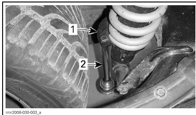
rmr2008-030-003_a REAR SUSPENSION ADJUSTMENT LOCATION
