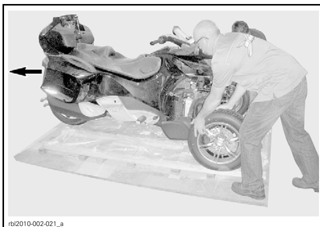
TYPICAL (RT MODEL SHOWN)
