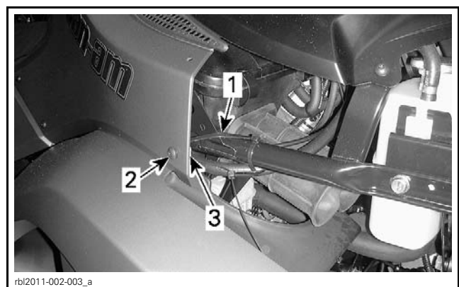
1. Locking tie 2. Front panel screw 3. Panel nut
