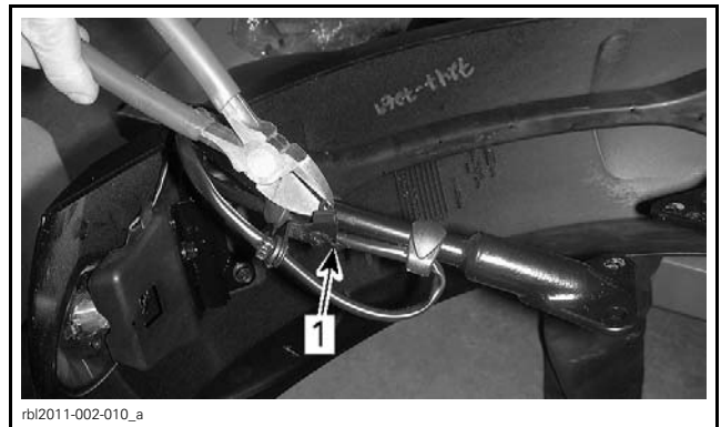
1. Locking tie
