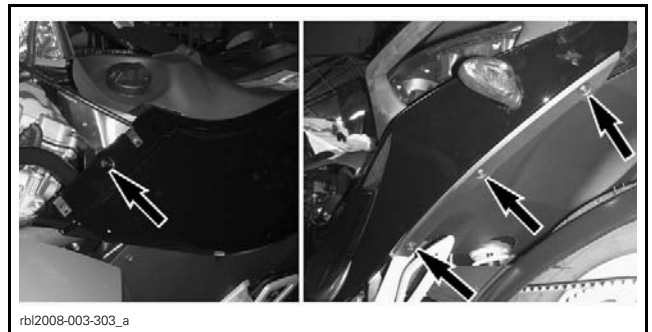
1. Retaining screws
