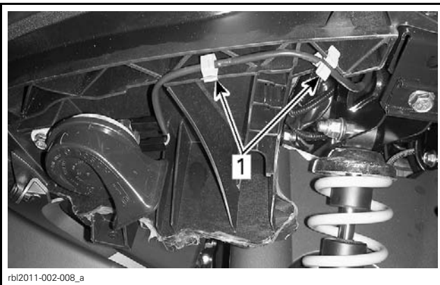
1. Cable retaining clips
