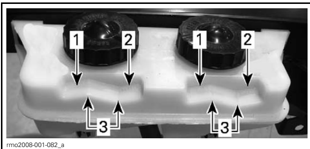
1. Brake fluid MAX. level mark 2. Brake fluid MIN. level mark 3. Operating range
