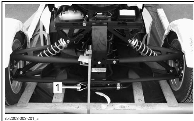
1. Front straps
