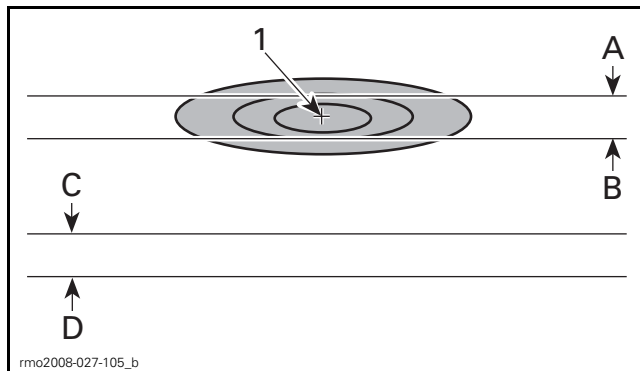
HEADLIGHT REFLECTION ON TEST SURFACE — HIGH BEAM
