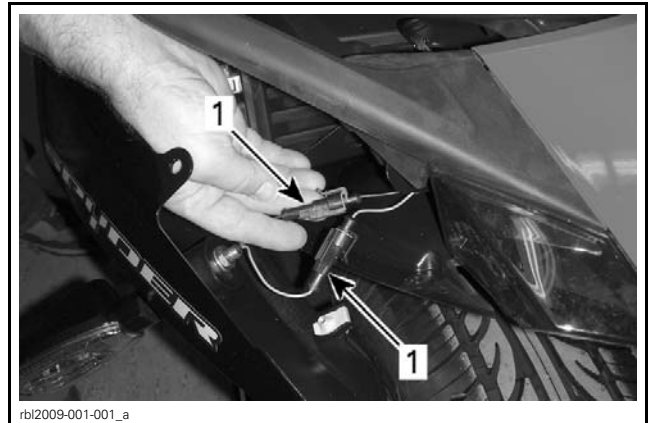
1. Turn signal connectors
