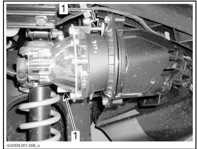
1. Adjustment screws
