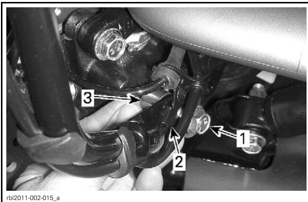
1. M8 x 35 hexagonal flange screws 2. Sleeves (one hidden) 3. Harness bracket
