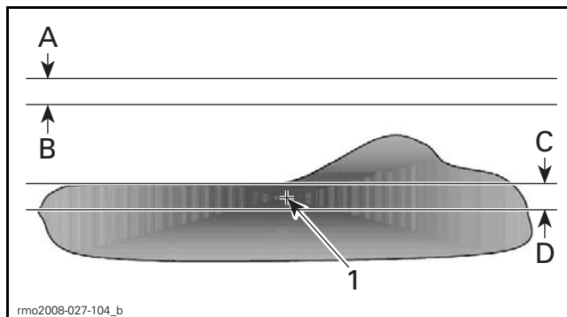
RH TRAFFIC HEADLIGHT REFLECTION ON TEST SURFACE — LOW BEAM
