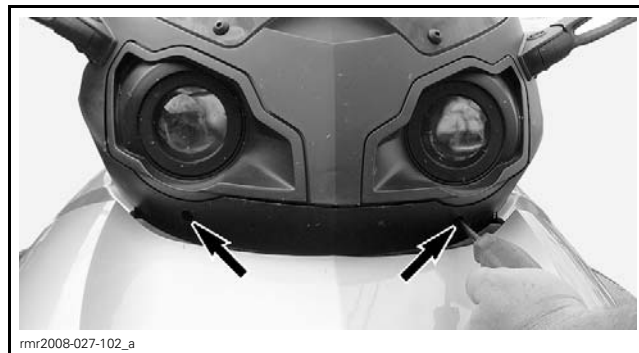
ADJUSTMENT SCREWS
