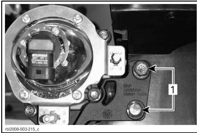
1. Retaining screws
