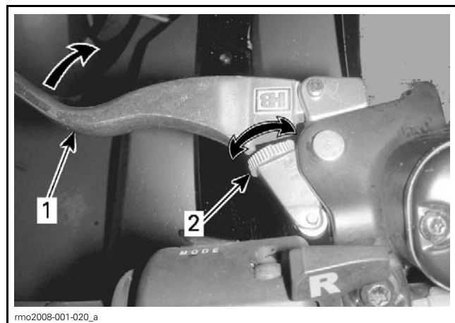
CLUTCH LEVER ADJUSTMENT
