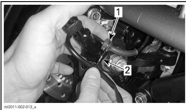
1. Cable grommet 2. Harness bracket
