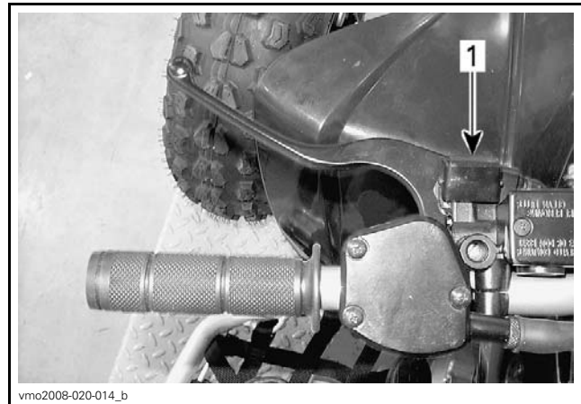
DS 90 X LH BRAKE LEVER 1. Parking brake mechanism
