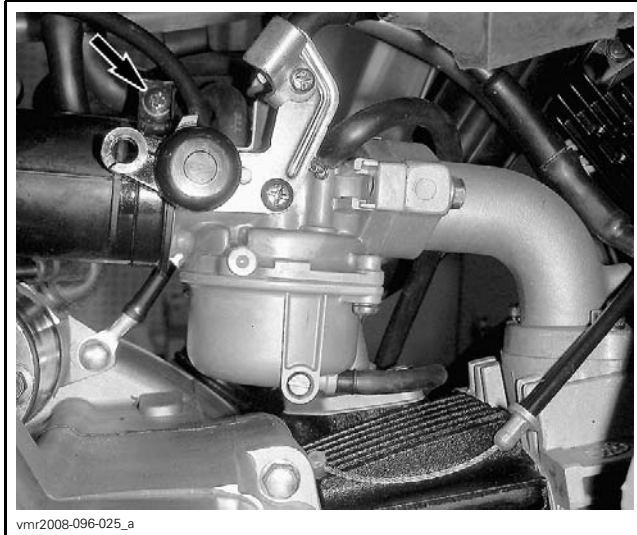
CARBURETOR BOOT CLAMP SCREW
