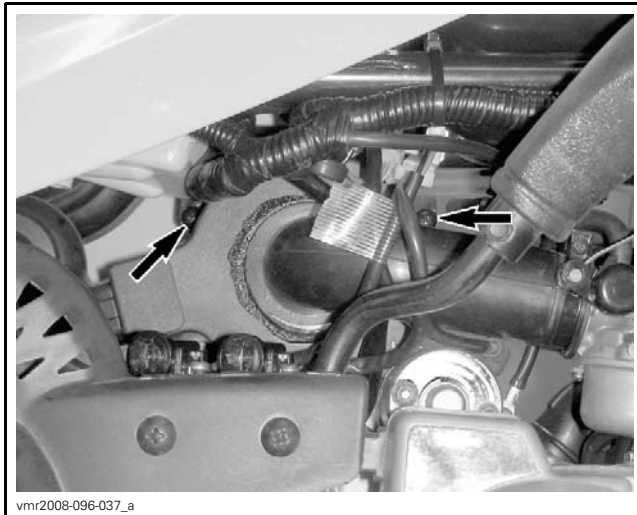
AIR FILTER HOUSING RETAINING SCREWS
