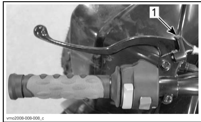
DS 70 AND DS 90 LH BRAKE LEVER 1. Parking brake mechanism
