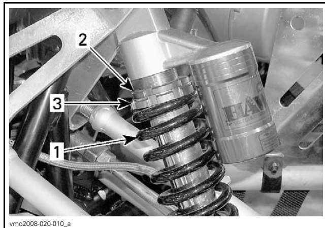
DS90 X FRONT SUSPENSION 1. Front spring 2. Locking ring 3. Adjustment ring
