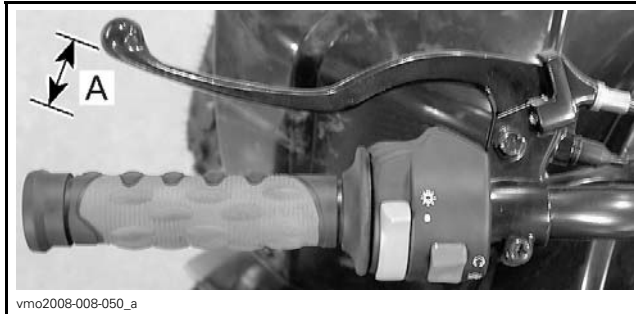
CABLE FREE-PLAY A. 15 mm to 25 mm (.6 in to 1 in)
