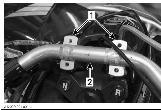
1. Lower supports 2. Handlebar
