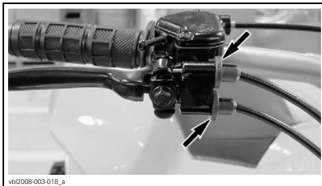
FRONT BRAKE LEVER ADJUSTING SCREWS
