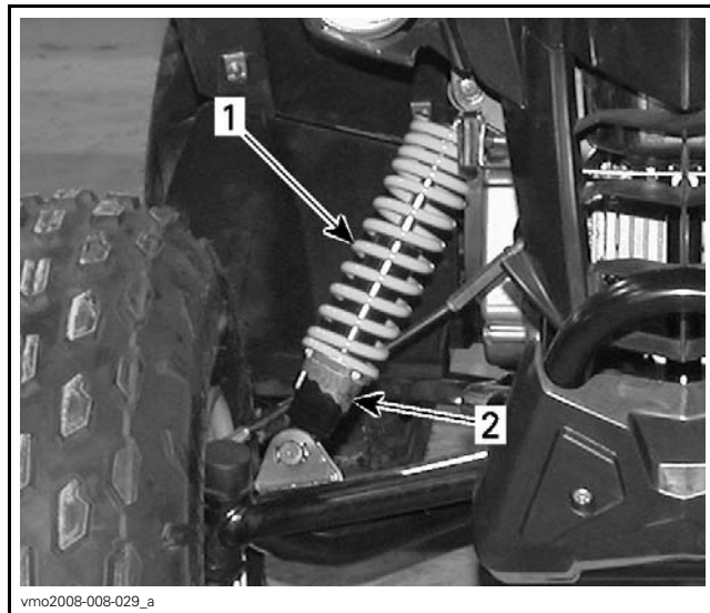
DS 70 AND DS 90 FRONT SUSPENSION 1. Front spring 2. Adjusting cam
