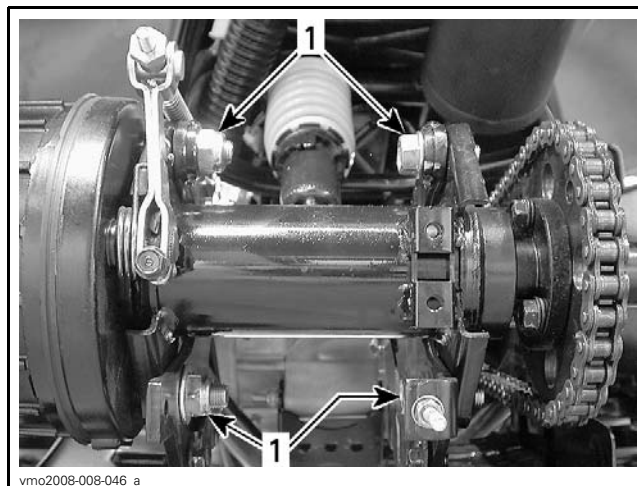
TYPICAL - REAR AXLE 1. Locking bolts
