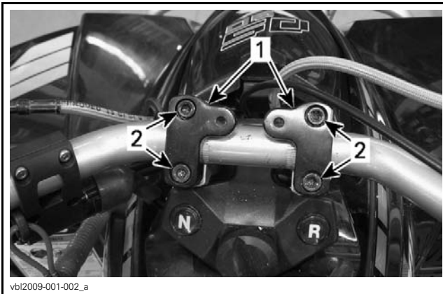
1. Upper supports 2. Handlebar retaining screws
