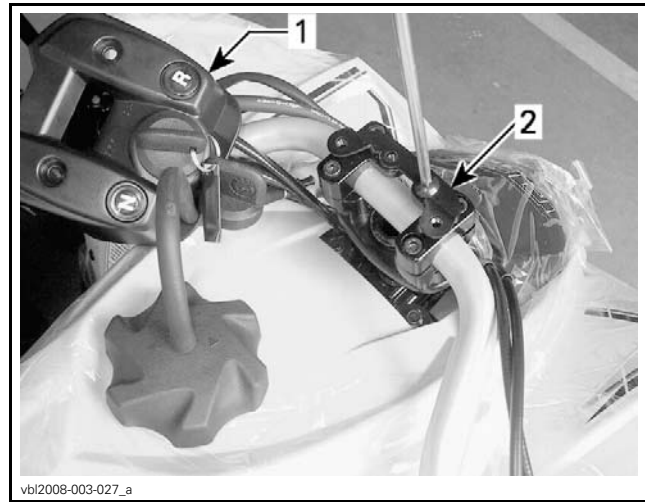
1. Center handlebar cap 2. Handlebar bracket
