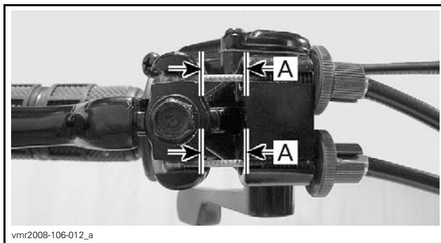
CABLE FREE-PLAY
