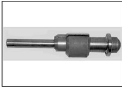
Piston circlip installer P/N 529 035 921 Mandatory 330, 400, 500, 650, 800 engines
