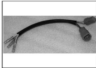
4-pin magneto diagnostic harness
