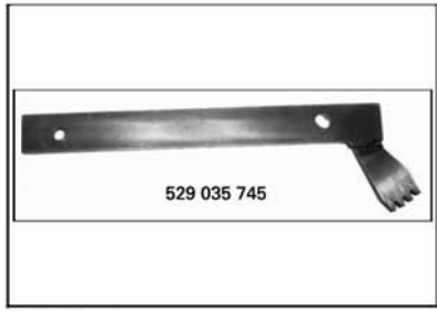
Clutch holder P/N 529 035 745 Recommended 610/500 engines
