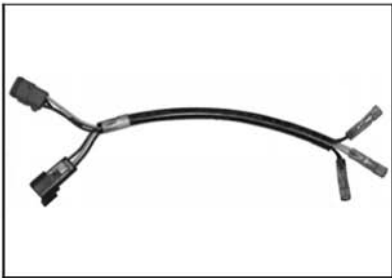
3-pin magneto harness adapter
