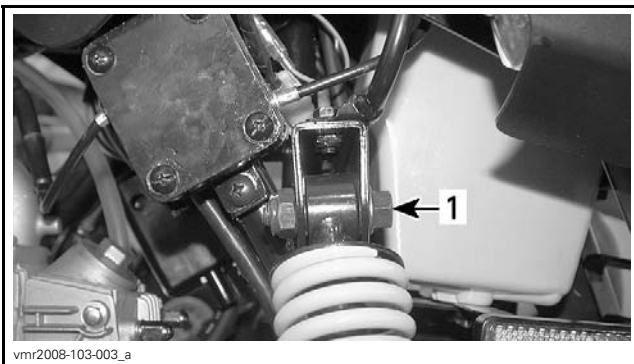
1. Upper bolt of shock absorber
