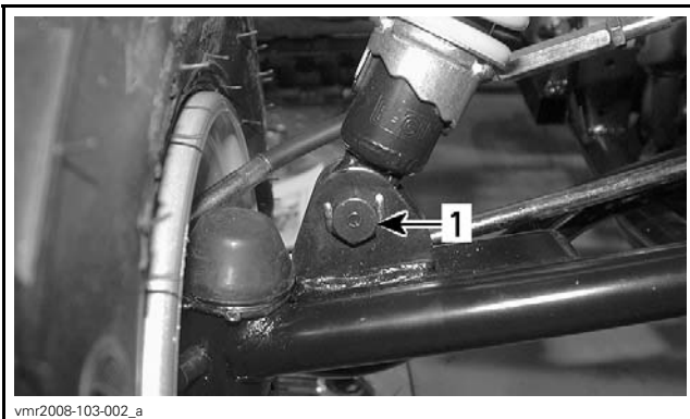
1. Lower bolt of shock absorber
