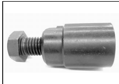
Flywheel puller P/N 529 035 792 Recommended DS 50/90, MY 2002-7
