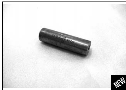
Valve guide installer (6 mm) P/N 529 036 075 Recommended 449, 991 engines Valve guide insertion jig
