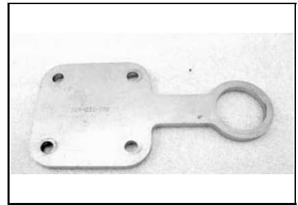
Engine lifting ring P/N 529 035 770 Recommended Quest 610/500
