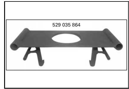
Clutch holding tool P/N 529 035 864 Recommended Rally 200 & DS 250
