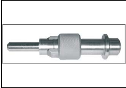
Piston circlip installer P/N 529 036 058 Recommended V-490 engine
