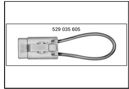
529 035 605 Wire jumper P/N 529 035 605 Recommended Traxter
