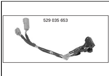
529 035 653 T harness P/N 529 035 653 Recommended Traxter To check shifting.
