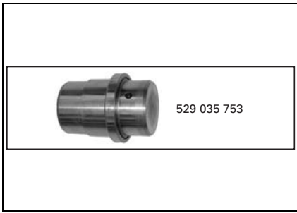
Crankshaft bearing puller P/N 529 035 753 Recommended 610/500 engines
