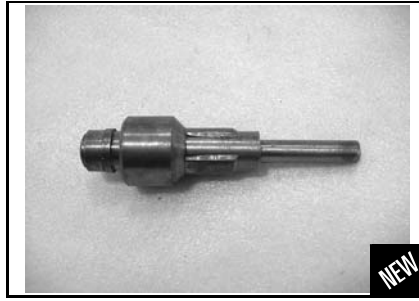
Piston circlip installer P/N 529 036 083 Mandatory 449 engine
