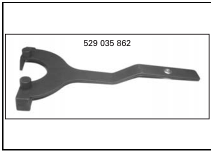
Clutch holding tool P/N 529 035 862 Recommended Rally 200
