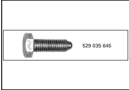
Crankshaft locking bolt P/N 529 035 645 Recommended Traxter 500
