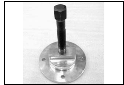
Hub puller P/N 529 035 612 Recommended
