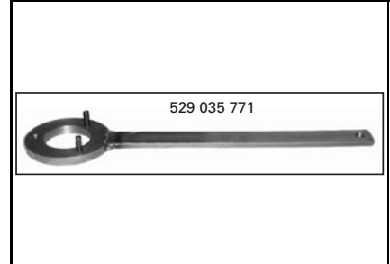
Driven clutch holder P/N 529 035 771 Recommended 330/400, 610/500, V-490, V-660, V-810
