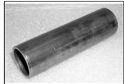
Crankshaft bearing installer (MAG) P/N 529 035 980 Recommended 552, 593HO, 693, 793 engines
