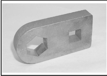
A-arm nut wrench P/N 529 035 876 REV, RT
