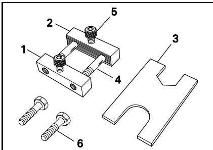
M10 bolt (item 4) P/N 222 007 565 Recommended All except Élan Part of kit 861725700
