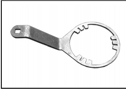
Fuel pump nut tool P/N 529 035 899 Recommended 2-TEC SDI and 4-TEC engines
