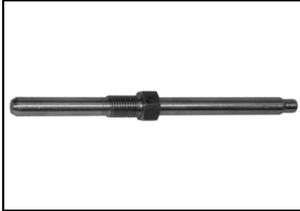
Crankshaft locking tool P/N 529 035 821 Recommended 4-TEC 1503 engines
