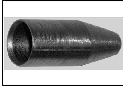
Oil seal guide P/N 529 035 822 Recommended 4-TEC 1503 engines
