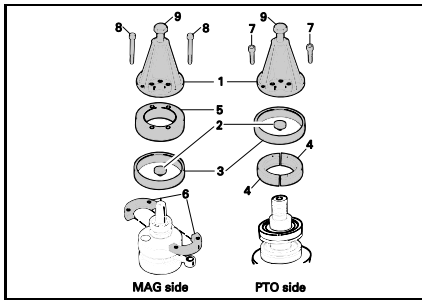
Puller ring P/N 420 977 490 Recommended 717/787 RFI engines
