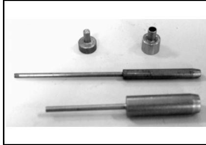
Needle jet height tool kit P/N 590 122 400 Recommended TM-40 carburetor, 2002 and 2003
