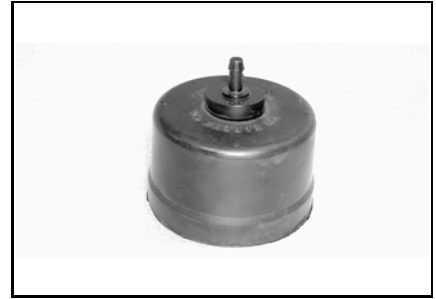
Manifold plug 63 mm (2-1/2") P/N 529 035 961 Recommended All 2-stroke engines Replacement part for item included in kit 861749100
