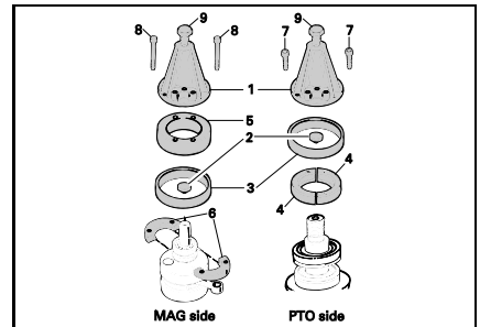
Distance ring (item 14) P/N 529 035 964 Recommended 693, 793 To be used with 420877635, for MAG side bearing
