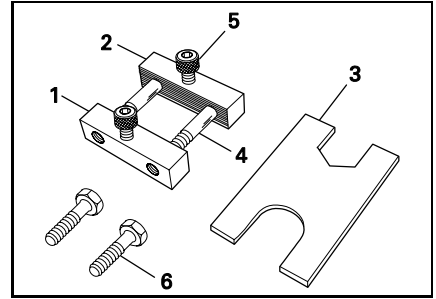
Block with threads (item 1) P/N 529 010 700 Recommended All except Élan Part of kit 861725700
