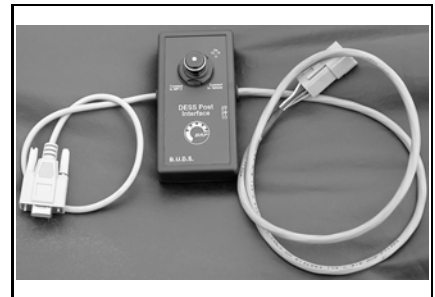
D.E.S.S. post interface P/N 529 036 019 Mandatory To programm D.E.S.S. keys with the MPI-2.
