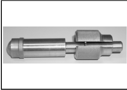
Piston circlip installer P/N 529 035 686 Mandatory All engines with tab type circlip
