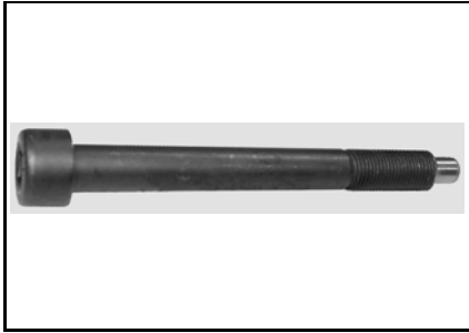
Crankshaft locking tool P/N 529 035 900 Recommended V-1000, V-1300
