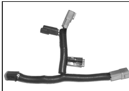
T-harness P/N 529 035 869 Mandatory All D.E.S.S. equipped
