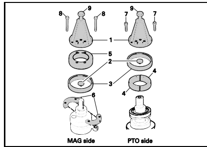
Puller ring P/N 420 977 494 Recommended 599, 699, 779, 809 Crankshaft bearing installer
