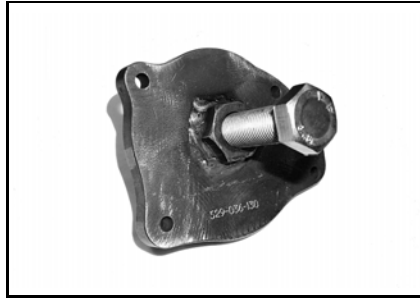
Ceramic seal pusher plate P/N 529 036 130 Recommended V-490, V-660 and V-810 engines Use with ceramic seal installer 529035766
