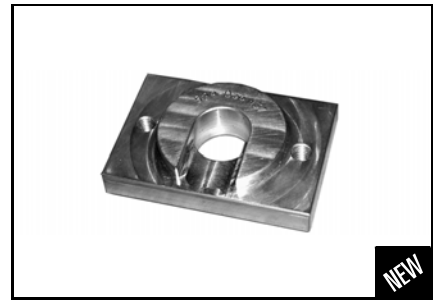
Injector retainer plate P/N 529 036 137 Recommended E-TEC
