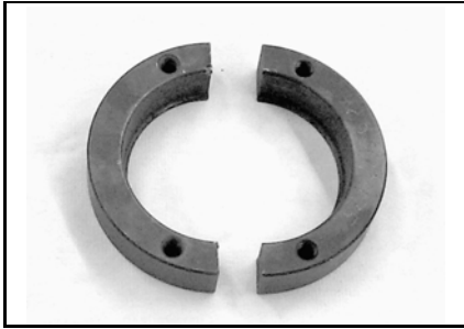
Half-ring puller P/N 420 876 330 Recommended 947 and 947 DI engines To remove 52 mm O.D. bearings from the crankshaft.
