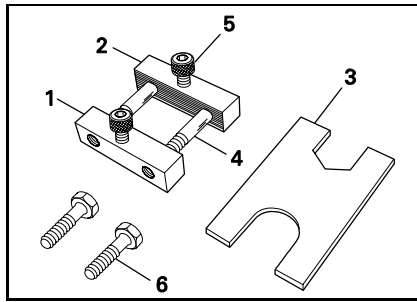
Drive axle sprocket adjuster kit
