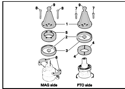
Half-rings P/N 420 977 479 Recommended 599, 699, 779, 809 3 cylinders crankshaft bearing remover; to use with 420877635
