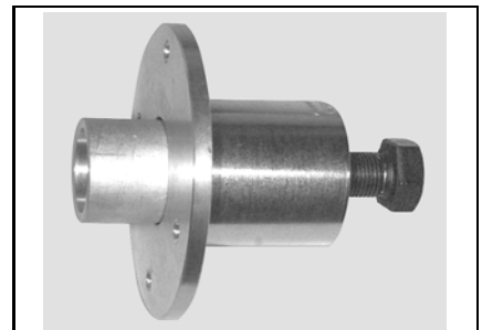
Ceramic seal pusher P/N 420 877 820 Recommended 494 and 670
