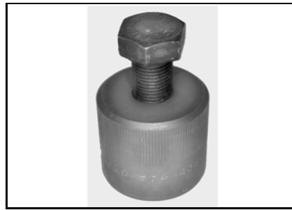
Flywheel puller P/N 420 976 235 Recommended 247, 787, 787 RFI, 947 and 947 DI eng. Replacement bolt P/N 529 035 549.
