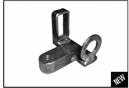
Engine lifting tool P/N 529 036 131 Mandatory E-TEC
