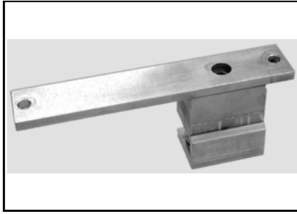
Belt tensioner tool P/N 529 035 957 Recommended Elite
