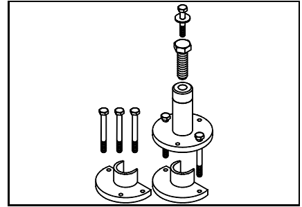
Countershaft bearing remover/installer P/N 529 035 699 Recommended REV, RT, ZX and CK3 Replaces 529035554.
