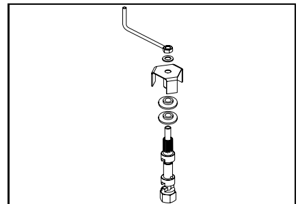
Replacement part for puller P/N 529 035 588 Recommended For 529036012
