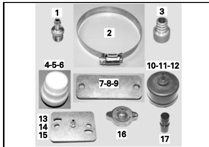
Intake plug (item 6) P/N 529 035 963 Recommended All 2-stroke engines Replacement part for item included in kit 861749100
