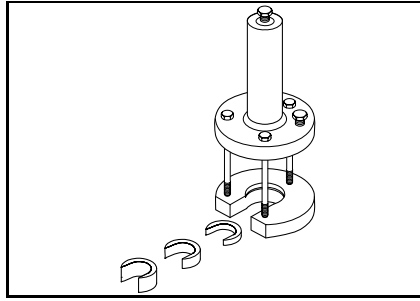
Countershaft bearing remover P/N 529 030 100 Recommended F and S series
