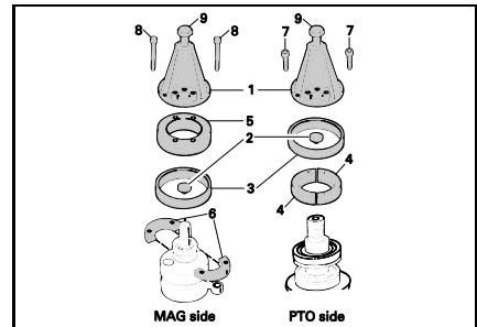
M8 x 40 screw (item 7) P/N 420 840 681 Recommended All 2-stroke engines
