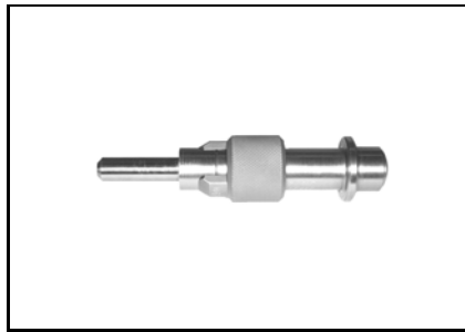
Piston circlip installer P/N 529 035 765 Recommended 610/500/1503/V-1000 engines
