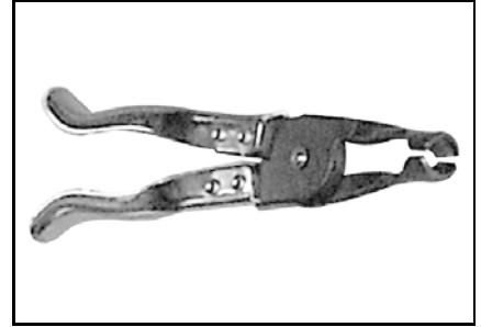
Valve stem seal removal pliers P/N Snap-on YA 8230 Recommended 1503, 991 engines, DS650 Not sold by BRP
