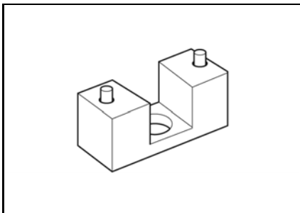
Spring cover puller P/N 529 027 300 Recommended Bombardier Lite
