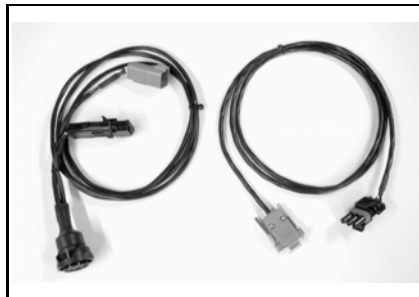
Handheld MEM programmer cable P/N 529 035 993 Recommended 6 pin connector.
