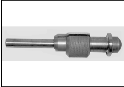
Piston circlip installer P/N 529 035 921 Mandatory 330, 400, 500, 650, 800 engines
