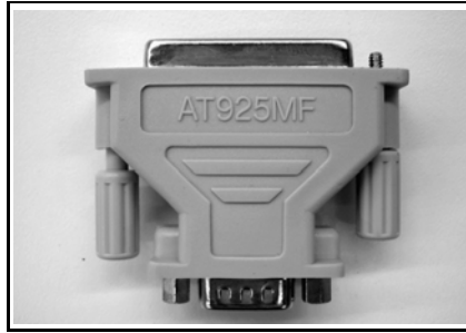
9 pins to 25 pins adaptor P/N 529 035 681 Recommended To connect communication cable P/N 529 035 697 of MPI to older PC.
