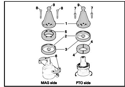
Crankshaft protector (item 2) P/N 420 976 890 Recommended 247 engine
