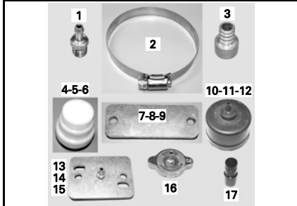
Replacement rubber seal (item 13) P/N 529 021 302 Recommended Replacement part for kit 861749100
