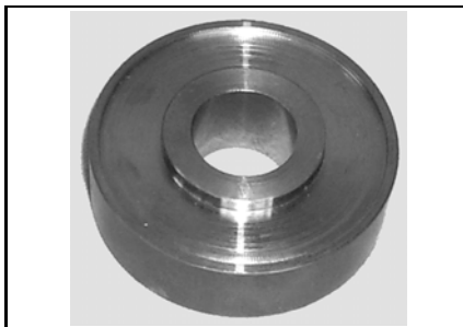
Engine support bearing installer P/N 529 035 952 Recommended Elite
