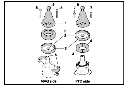
Holder ring (item 3) P/N 420 977 480 Recommended 947DI engines
