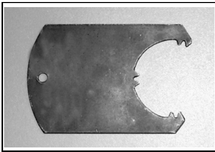
Gear holder P/N 420 876 695 Recommended 277F, 377F, 447 and 503 To hold the oil pump gear
