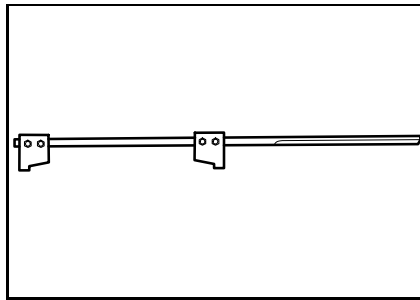
Pulley alignment bar P/N 529 035 545 Recommended 1998 Skandic WT
