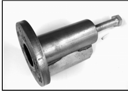
Crankshaft bearing puller P/N 529 036 004 Recommended 2-stroke engines
