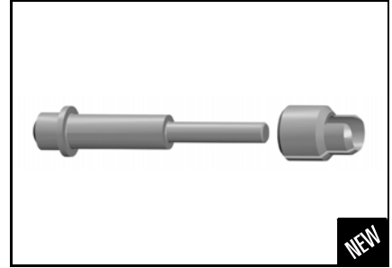
Piston circlip installer P/N 529 036 153 Recommended 1203
