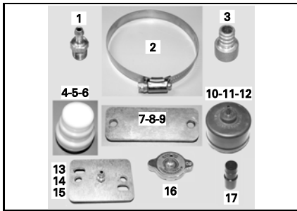
RAVE plate (item 8) P/N 529 035 971 Recommended All 2-stroke engines Replacement part for item included in kit 861749100
