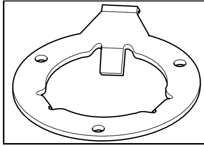
Fan holder wrench P/N 420 876 357 Mandatory All axial fan engines Except 552F
