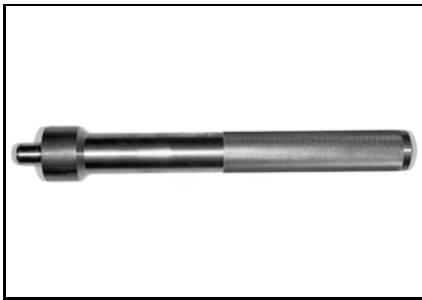
Rotary valve bearing pusher P/N 420 876 501 Recommended 717, 787 and 787 RFI engines
