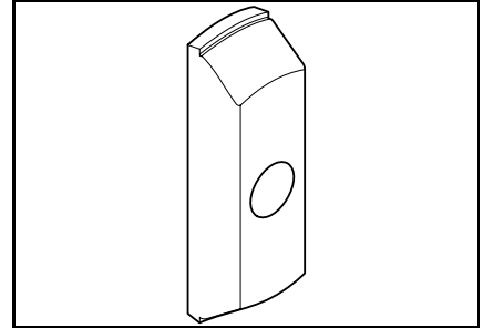
Large bushing extractor P/N 529 035 576 Recommended Formula type driven pulley To be used with 529035524
