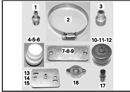
Intake plug (item 5) P/N 529 030 500 Recommended All 2-stroke engines Replacement part for item included in kit 861749100
