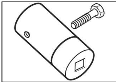
Drive pulley puller P/N 529 023 100 Recommended Elan
