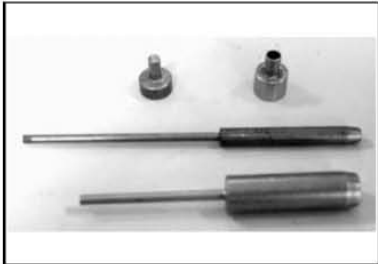
Needle jet height tool kit P/N 590 122 400 Recommended TM-40 carburator, 2002 & 2003
