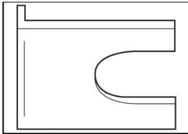
Crankshaft feeler gauge P/N 420 876 620 Recommended 377, 443, 447 & 503
