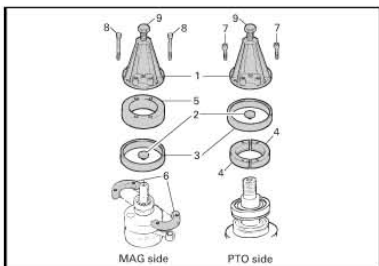
Screw M8x70 (item #8) P/N 420 841 201 Recommended All 2-stroke engines To be used with P/N 827 635.
