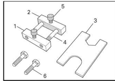
Drive sprocket position adjuster kit
