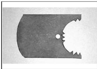
Gear holder P/N 529 036 061 552 Fan To hold oil pump gear.
