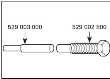
Drive pulley puller
